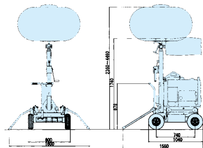
LB1130FBD-1
